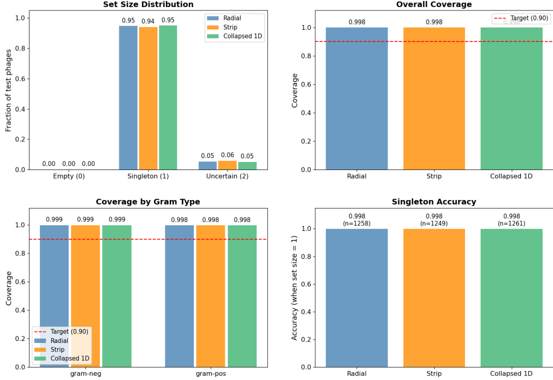
Figure 5.1: Gram type classification performance across Radial, Strip, and Collapsed 1D geometries on the test split (Split 0, target 1 - \alpha = 0.90 ). Panels show: (top-left) prediction set size distribution, (top-right) marginal empirical coverage, (bottom-left) class-conditional coverage, and (bottom-right) singleton accuracy with sample counts ( n ).
